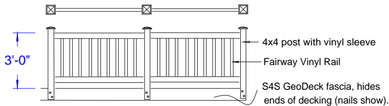
Standard Fairway Vinyl Railing Detail
