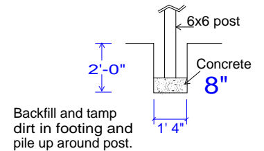
Typical F6 Footing
