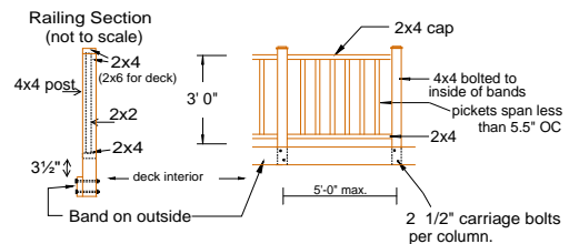
Detail for GeoDeck Railing Bolted to INSIDE of Gazebo, Deck or Porch Floor
