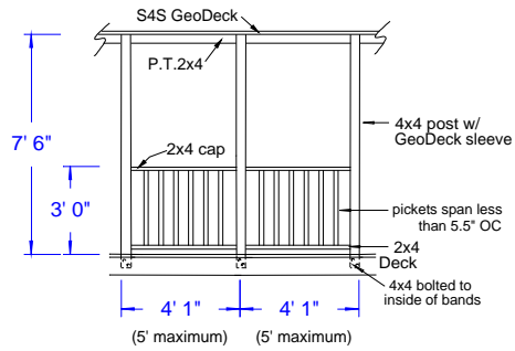
A to B Planter Wall Detail
