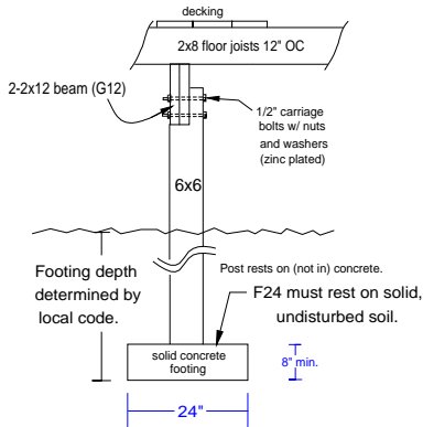
Typical Spa Substructure
